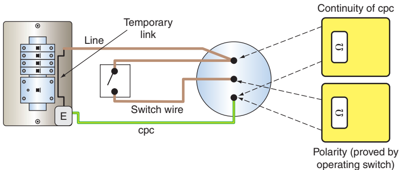
FIGURE 6.8 Lighting polarity.
