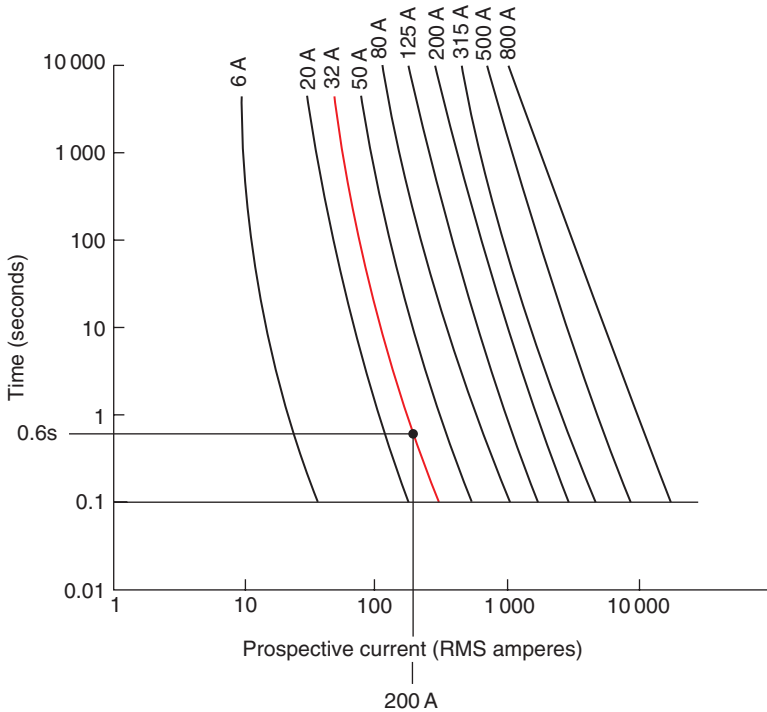
FIGURE 5.9 Time/current characteristics for fuses to BS 88 Part 2. Example for 32A fuse superimposed.
