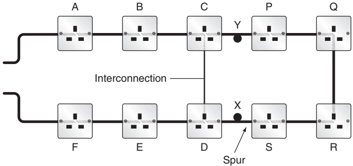
FIGURE 6.3 Ring circuit with interconnection.
