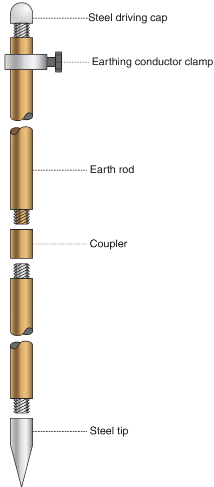
FIGURE 2.3 Earth rod.
